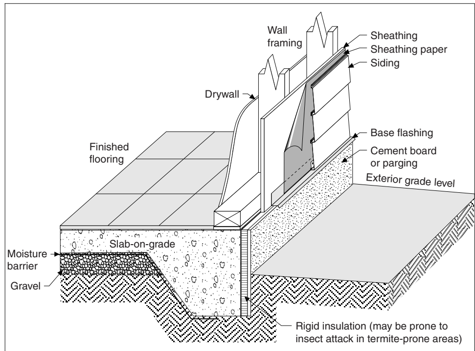
FIGURE 1.8 Slab-on-Grade—Monolithic Slab
